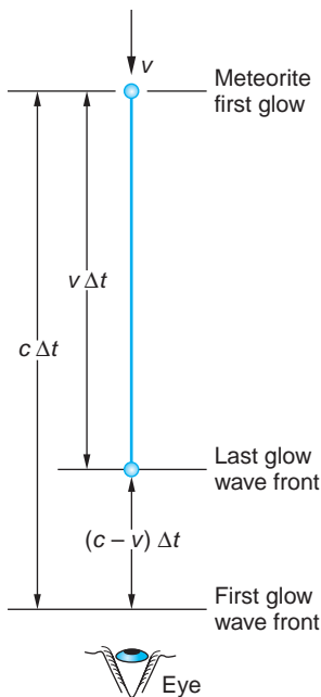
FIGURE 1-40 A meteorite moves directly toward the observer’s eye at speed v . The spatial distance between the wave fronts is (c - v)\Delta t as they move at c , so the time interval between their arrival at the observer is not \Delta t , but \Delta t_{\text{eye}} , which is (c - v)\Delta t / c = (1 - \beta)\Delta t , and the apparent speed of approach is v_a = v\Delta t / \Delta t_{\text{eye}} = \beta c / (1 - \beta) .
